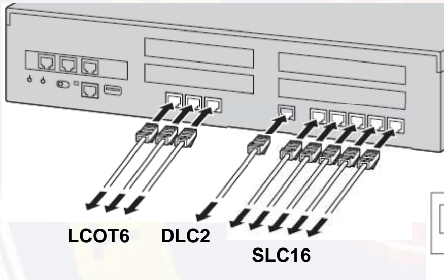
Main cabinet
