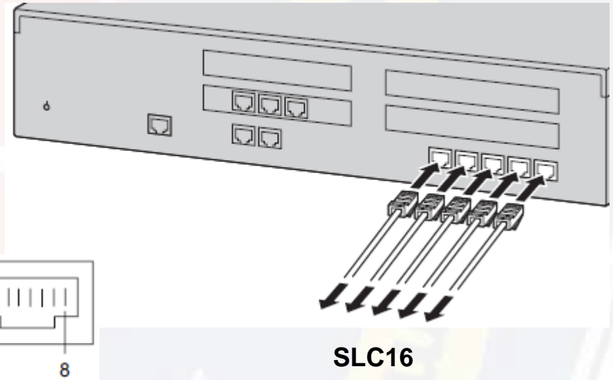
Expansion Cabinet
